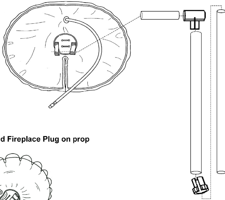
Fig 1: Assemble prop and Fireplace Plug as shown
